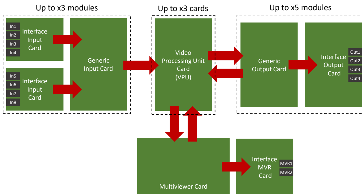
Figure 1: Simplified block diagram of the LivePremier architecture
